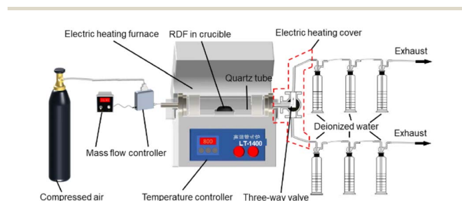
Fig. 2 Experimental system of RDF combustion and gaseous chlorine collection.
