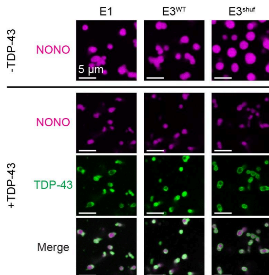
Fig. S8. TDP-43 opposes NONO condensation by forming surfactant-like layers on condensate surfaces. Confocal slices of condensates assembled with 2 \mu M NONO (magenta) + 15 nM of the indicated RNAs \pm 0.2 \mu M TDP-43 (green) after 3 h at 25 ^{\circ} C. NONO and TDP-43 channels are each contrasted equally across all images.
