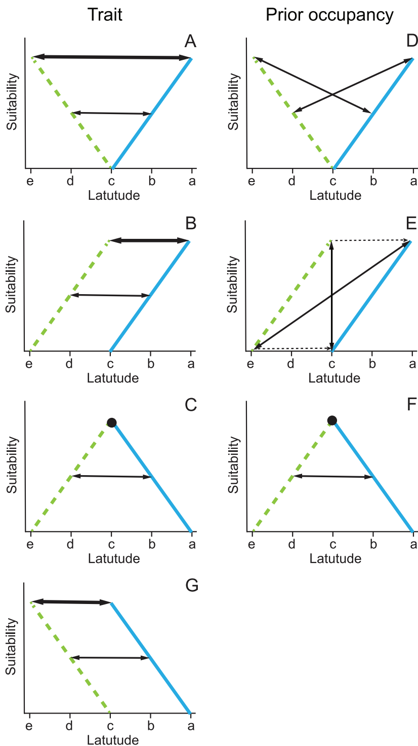
Figure 2. Illustrations of suitability gradients as a function of latitude with migration cost included for different evolutionary scenarios, under which chain or leapfrog migration may evolve. Solid (blue) lines refer to breeding suitability (sites a-c), whereas broken (green) lines refer to winter suitability gradients (sites c-e). Filled (black) circle refer to resident population. Panels A-F refer to scenarios outlined in Holmgren and Lundberg (1993), with panels A-C referring to trait-related dominance, and panels D-F prior occupancy-related dominance. Leapfrog migration evolves under panels A, C, E, and F, whereas chain migration evolves under panels B and D. Panel G is a new situation considered here where dominance due to body size leads to chain migration. In panel G, dominant (large) birds will exclude subdominant (small) birds from the best breeding site (c), and after breeding they will migrate to the most favorable (e) site for wintering (upper arrow). Subdominants will be forced to adopt the b-d route (lower arrow), hence chain migration arise. Latitude a-e varies from north to south. For further information, see main text, and Holmgren and Lundberg (1993).
