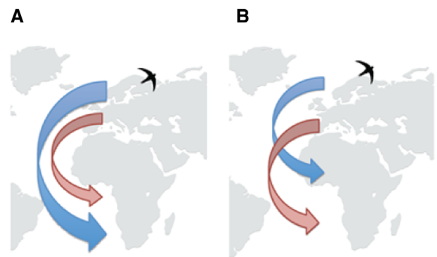
Figure 1. Schematic view of predicted typical migration patterns. (A) Leapfrog migration pattern and (B) chain migration pattern.
