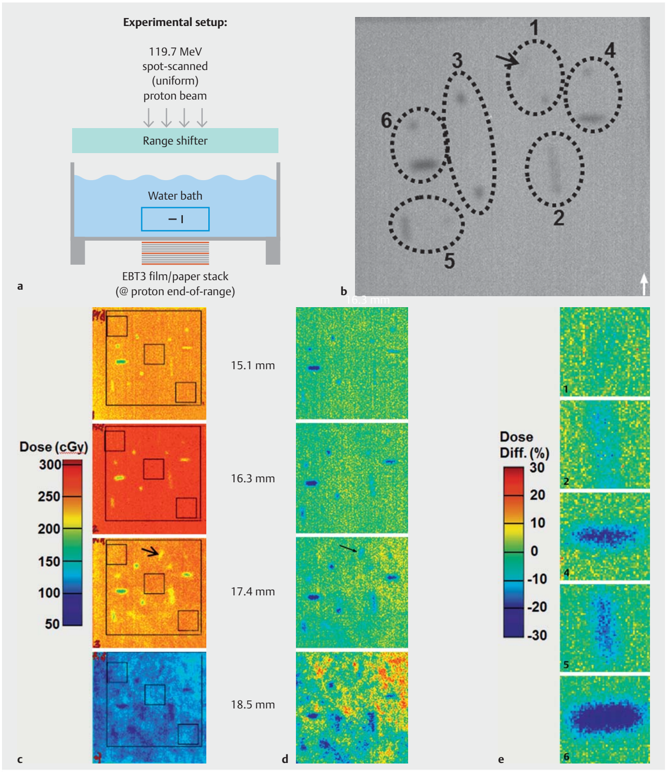
Fig. 1 a Schematic of experimental setup: a gel phantom containing fiducial samples was submerged in a water bath and irradiated with a uniform 10 \times 10 \text{ cm}^2 field of 119.7 MeV protons using discrete spot scanning. Exiting the water bath, the protons stopped in a paper stack arrangement interleaved with four EBT3 (Gafchromic) films spaced approximately 1.1 mm apart (water-equivalent spacing). b Digitized EBT3 film (16.3 mm behind fiducial plane, closest to the Bragg Peak) identifying the set of fiducial samples included in the present study. Note that an edge-on example for Sample 2 was not incorporated in the gel phantom. The side-on example for Sample 2 is difficult to visualize and therefore black arrows are included as a guide-to-eye (in b , c , and d ). c Dose in cGy for a set of EBT3 films exposed to the end-of-range region, with water-equivalent depths behind the fiducial plane as shown. The small ROIs indicate the regions used for nominal (or background) dose sampling (for normalization) and the large ROIs designate the cropping regions for d . d Dose difference (from background) in % for corresponding cropped film regions from c . e Dose differences observed nearest the Bragg Peak (16.4 \times 6.4 mm 2 ) for zoomed (6.4 \times 6.4 mm 2 ) ROIs affected by the five given side-on samples (#1, #2, #4–6).
