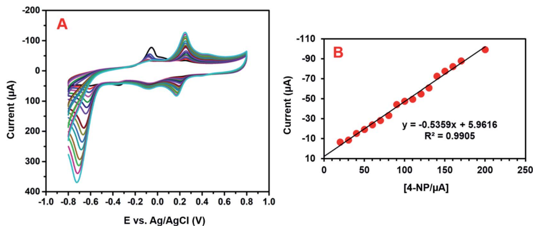
Fig. 9 (A) The obtained CV response for the GCE/CNF/CuCrO 2 electrode for the detection of 0.1 to 200 μM 4-NP in PBS. (B) Calibration plot between the peak current and concentration of 4-NP.
