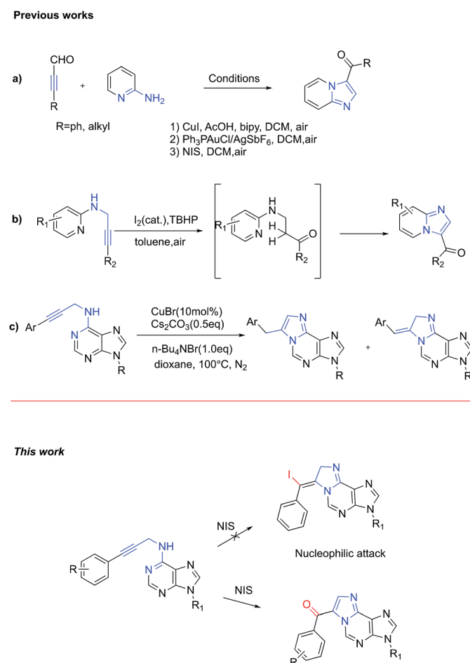
Scheme 1 Diverse constructions of imidazo[1,2- a ]pyridine.
