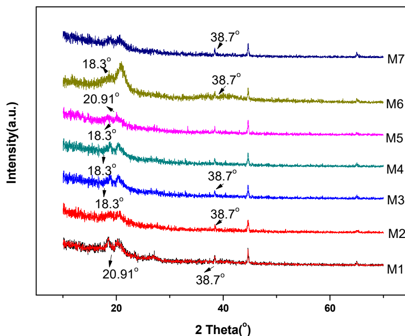
Figure 5. XRD spectra of nanocomposite membranes.
