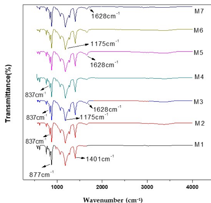
Figure 4. FTIR spectra of nanocomposite membranes.
