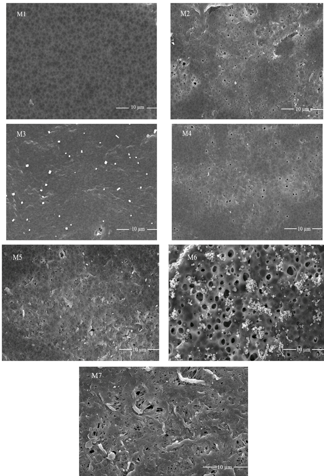
Figure 6. SEM analysis for the surface morphological studies of nanocomposite membranes: Top four membranes from the left named as M1 (PVDF only), M2 (PVDF-1% PVP), M3 (0.1% SGO), M4 (0.2% SGO) and bottom three as: M5 (0.3% SGO), M6 (0.4% SGO) and M7 (0.5% SGO).
