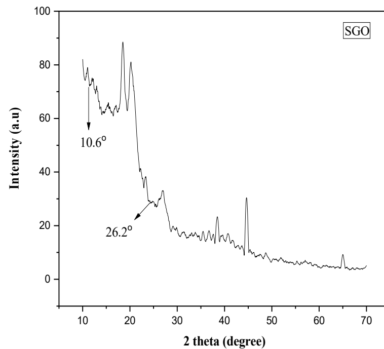
Figure 3. XRD spectrum of sulfonated graphene oxide.
