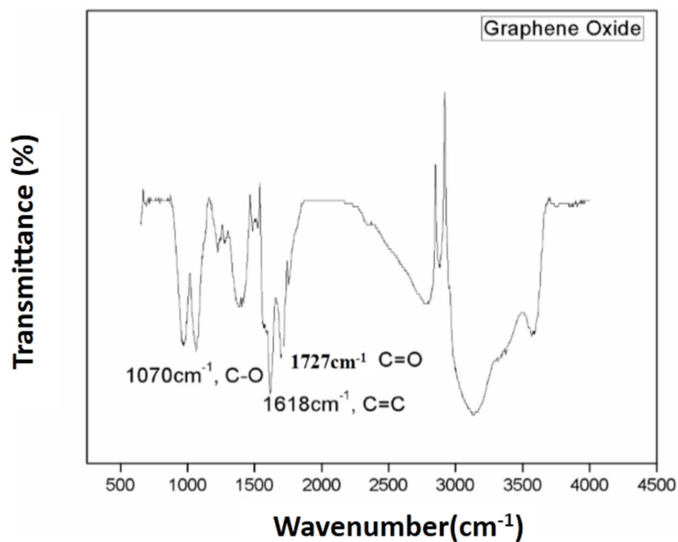
Figure 1. FTIR spectrum of graphene oxide.
