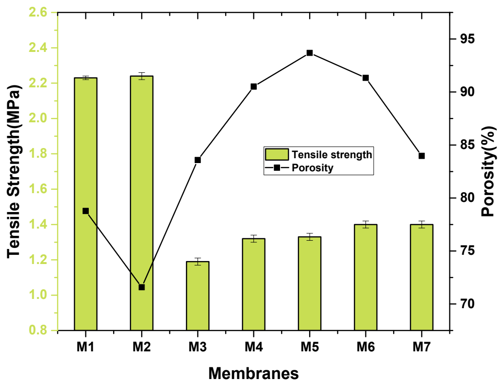
Figure 8. Porosity and tensile strength of nanocomposite membranes.
