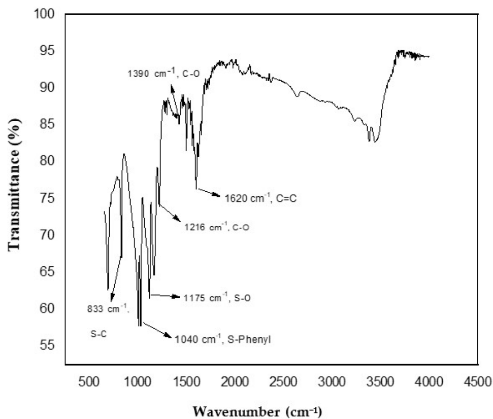
Figure 2. FTIR spectrum of sulfonated graphene oxide.
