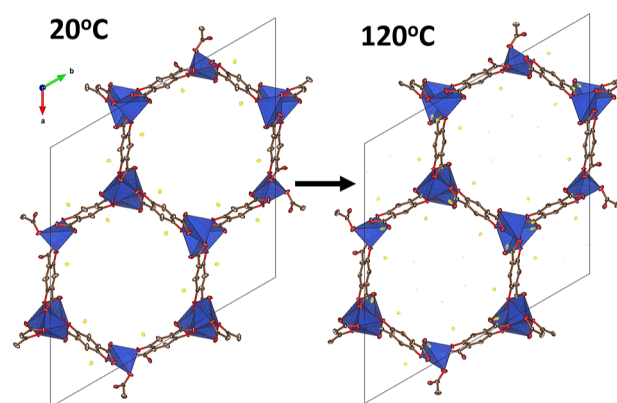
Figure 7. Dynamically refined structures of Cu-MOF-74 at Post SE (20 °C) and Post 120 °C, showing the remaining electrostatic potentials above 0.095 eV/Å 3 (2.3 \sigma ). The atoms are displayed as their displacement ellipsoids. C atoms are displayed in brown, O atoms in red, and Cu atoms in blue. The electrostatic potentials are displayed in yellow.
