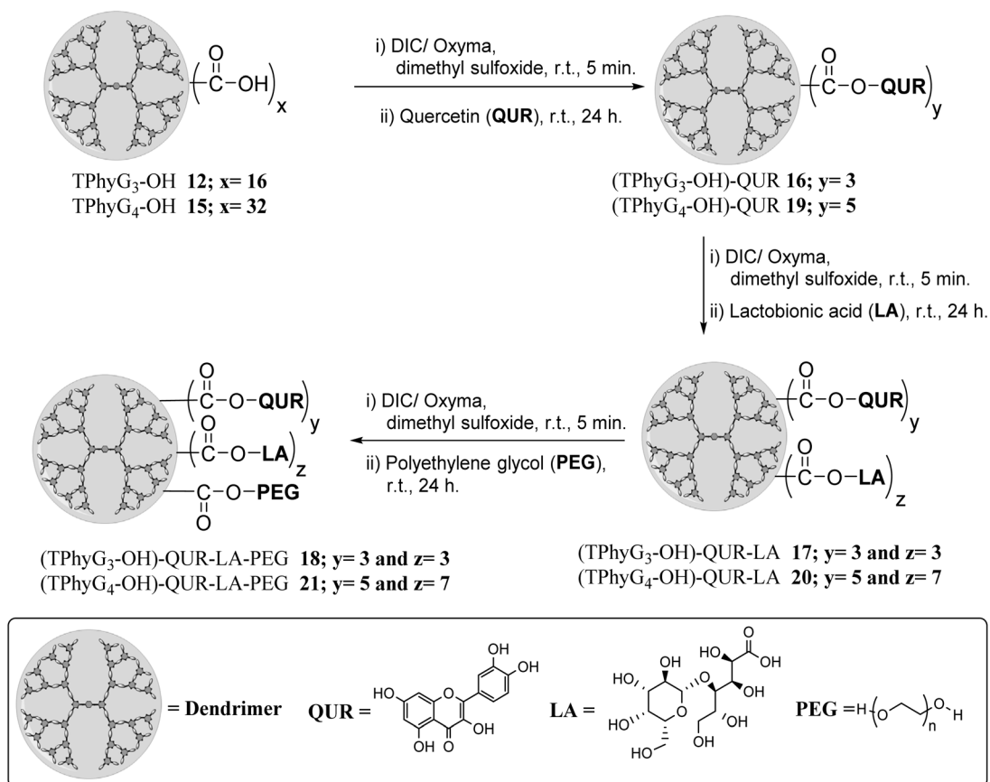
Scheme 6 Synthesis of PEGylated lactobionic acid-targeted Quercetin-dendrimer conjugates 18–21 .
