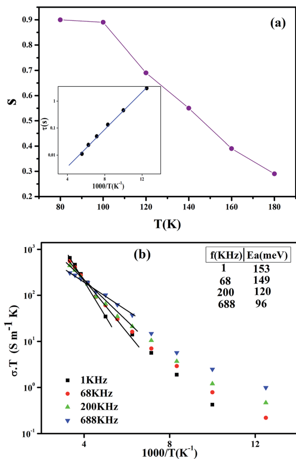
Fig. 6 (a) Temperature dependence of the frequency exponent s , the inset shows the plot of ' \tau ' versus 1000/T . (b) Arrhenius plot of (\sigma_{ac}T) at different frequencies for \text{Pr}_{0.65}\text{Ca}_{0.25}\text{Ba}_{0.1}\text{MnO}_3 .
