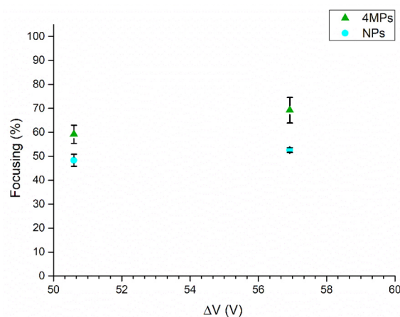
Figure 8. UV-Vis characterization of focusing performance of the BAW device when a mixed population of 4MPs concentrated at 2.84 \times 10^5 particles/mL and NPs concentrated at 1.82 \times 10^5 particles/mL was injected at 1 \mu\text{L}/\text{min} into the device, which was actuated at its resonance frequency of 4.623 MHz. Experiments were performed by applying 50.59 Vpp and 56.92 Vpp at the transducer.
