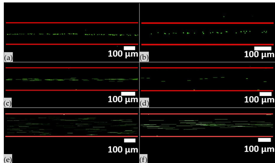
Figure 6. Frame of time lapse acquired during the acoustophoretic test, when 4MPs were employed at different concentrations and flow rates: (a) 4MPs concentrated at 5.68 \times 10^6 particles/mL were injected at 1 \mu\text{L}/\text{min} , (b) 4MPs concentrated at 1.41 \times 10^6 particles/mL were injected at 1 \mu\text{L}/\text{min} , (c) 4MPs concentrated at 5.68 \times 10^6 particles/mL were injected at 3 \mu\text{L}/\text{min} , (d) 4MPs concentrated at 1.41 \times 10^6 particles/mL were injected at 3 \mu\text{L}/\text{min} , (e) 4MPs concentrated at 5.68 \times 10^6 particles/mL were injected at 10 \mu\text{L}/\text{min} and (f) 4MPs concentrated at 1.41 \times 10^6 particles/mL were injected at 10 \mu\text{L}/\text{min} . Experiments were performed by applying 50.59 Vpp at the transducer, while the device was actuated at its resonant frequency of 4.623 MHz. Images acquired with 4\times objective lens with an exposure time of 9.8 ms.
