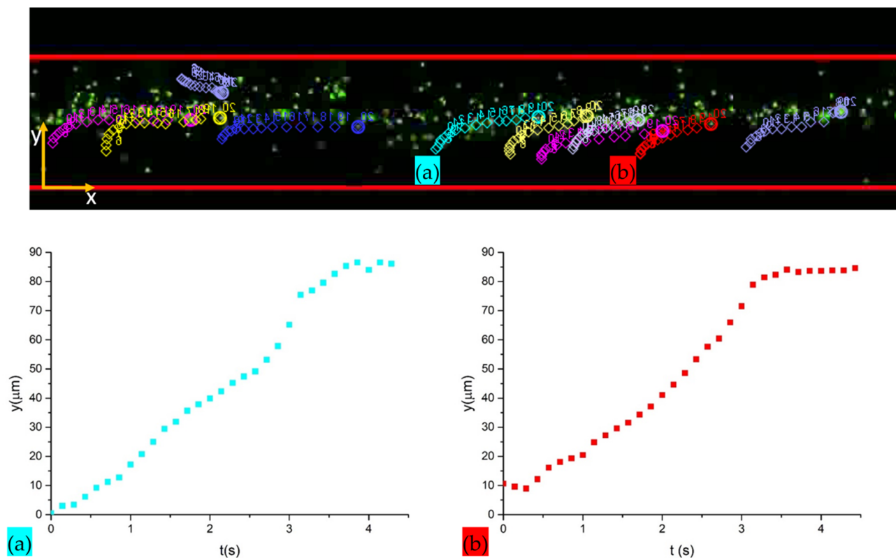
Figure 9. Tracking of bead paths with the Tracker 2.6 software and measurement of the transverse path y(t) from channel walls to the pressure node of two different beads (a) and (b). Measurements were performed in a specific focal plane of the 4\times objective lens of the fluorescence microscope.
