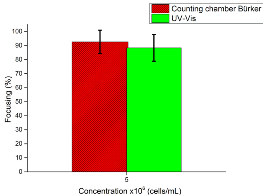
Figure 12. Focusing performance of the BAW device from Bürker counting chamber analysis and UV-Vis characterization. HL-60 cells concentrated at 5 \times 10^6 cells/mL were injected at 3 \mu\text{L}/\text{min} when 50.59 \text{ Vpp} was applied to the transducer, while the device was actuated at its resonance frequency of 4.623 \text{ MHz} .
