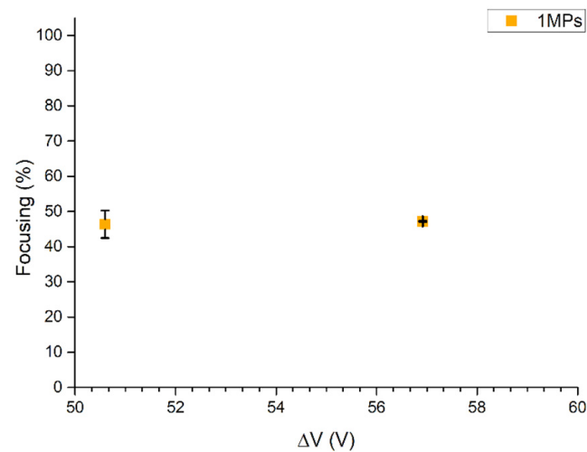
Figure 7. UV-Vis characterization of focusing performance of the BAW device with 1MPs concentrated at 1.00 \times 10^6 particles/mL injected at 1 \mu\text{L}/\text{min} when the device was actuated at its resonance frequency of 4.623 MHz. Experiments were performed by applying 50.59 Vpp and 56.92 Vpp at the transducer.
