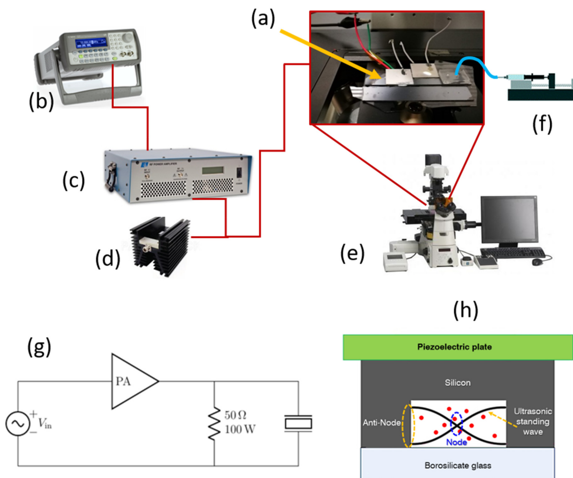
Figure 2. Experimental setup: (a) BAW device and resonating plate in which: the light blue line indicates the MP solution and the red one the electrical connections to actuate the piezoelectric elements (white), (b) waveform generator, (c) RF power amplifier, (d) dummy load, (e) optical fluorescence microscope, (f) syringe pump, (g) electrical diagram of the experimental setup used to generate the US standing wave into the microfluidic channel, (h) cross section sketch of the BAW device operating principle.
