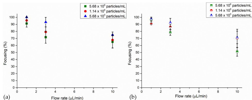
Figure 4. Focusing performance of the BAW device as a function of flow rates and 4MP concentrations: (a) UV-Vis characterization and (b) image analysis. Experiments were performed with 4MPs concentrated at 5.68 \times 10^6 particles/mL, 1.14 \times 10^6 particles/mL and 5.68 \times 10^5 particles/mL. During the experiments, 4MPs were injected at 1 \mu\text{L}/\text{min} , 3 \mu\text{L}/\text{min} and 10 \mu\text{L}/\text{min} , while 50.59 Vpp was applied at the transducer when the device was actuated at its resonant frequency of 4.623 MHz.
