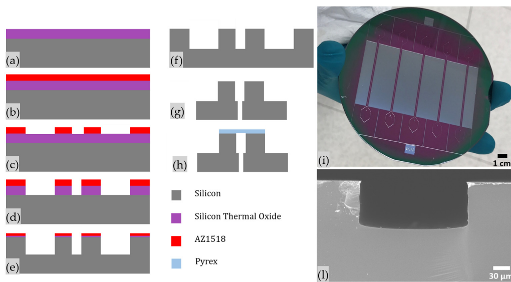
Figure 1. Chip Process Flow: (a) starting substrate cleaning, (b) photoresist spin coating, (c) photoresist exposure and development, (d) buffer oxide etching, (e) silicon deep reactive ion etching, (f) buffer oxide etching, (g) inlet/outlet laser drilling and chip dicing, (h) anodic bonding, (i) BAW devices after DRIE process and (l) Field Emission Scanning Electron Microscope (FESEM) cross section image of the separation channel.
