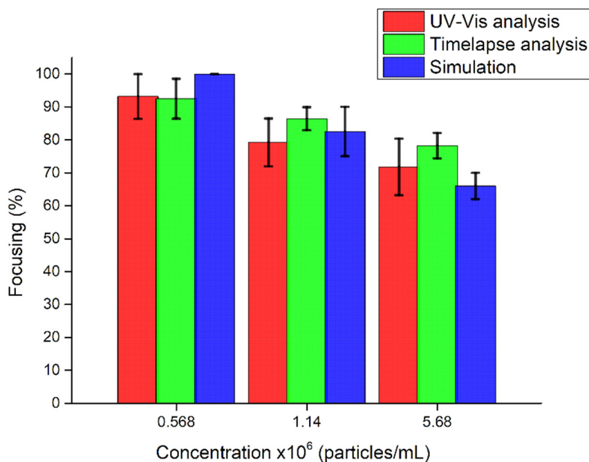
Figure 10. Comparison of the focusing performance of the BAW device obtained through simulations and experiments when 4MPs at different concentrations ( 5.68 \times 10^6 particles/mL, 1.14 \times 10^6 particles/mL and 5.68 \times 10^5 particles/mL) are investigated. Experimental values are reported, characterized either by UV–Vis analysis or image analysis.
