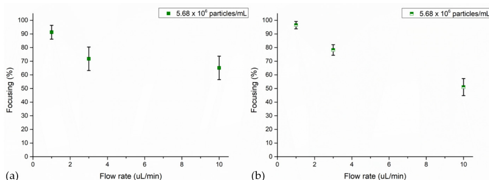
Figure 3. Focusing performance of the BAW device with 4MPs concentrated at 5.68 \times 10^6 particles/mL injected at 1 \mu\text{L}/\text{min} , 3 \mu\text{L}/\text{min} and 10 \mu\text{L}/\text{min} : (a) UV–Vis characterization and (b) image analysis. Experiments were performed by applying 50.59 Vpp at the transducer while the device was actuated at its resonant frequency of 4.623 MHz.
