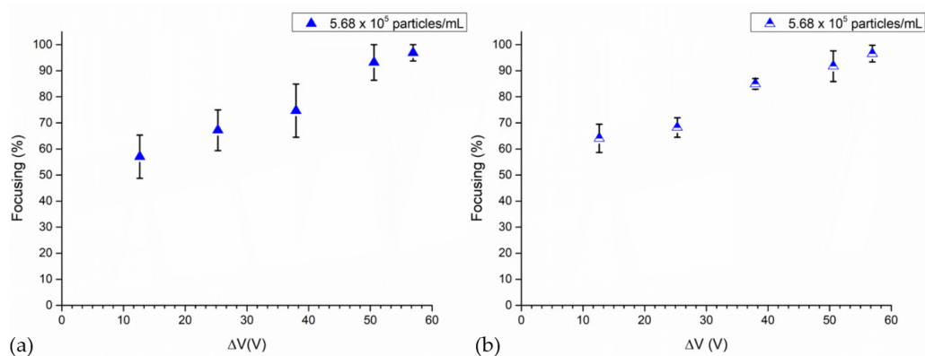
Figure 5. Focusing performance of the BAW device as a function of applied voltages at the transducer: (a) UV-Vis characterization and (b) image analysis. During the experiments, 4MPs concentrated at 5.68 \times 10^5 particles/mL were injected at 3 \mu\text{L}/\text{min} into the device actuated at its resonant frequency of 4.623 MHz, while 56.92 Vpp, 50.59 Vpp, 37.95 Vpp, 25.29 Vpp and 12.65 Vpp were applied at the transducer.
