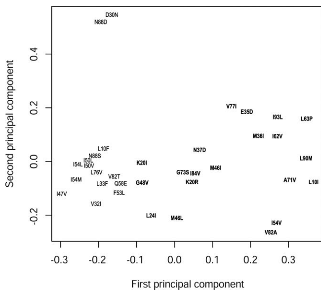
Figure 1. Multidimensional Scaling of 35 HIV-1 Protease Mutations
