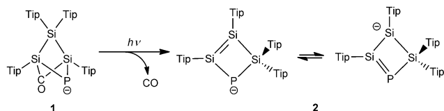
Scheme 2. Photolysis of 1 to afford 2 .
