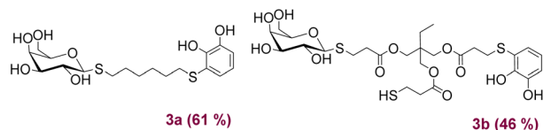
Fig. 2 Structure and yields of products 3 obtained after deprotection of 2.
