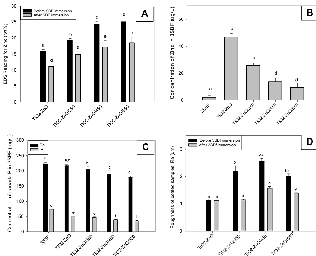
Figure 3 The effect of heat treatment on the composition and the leaching of \text{TiO}_2\text{-ZnO} coating during the synthesis of the composite coating. (A) The total concentration of zinc on the differently heat treated \text{TiO}_2\text{-ZnO} discs before and after exposure to 3SBF by EDS analysis. (B) The total concentration of zinc in the 3SBF measured by ICP-MS after 24-hr exposure. (C) The concentration of total calcium and phosphorus in the 3SBF measured by ICP-MS after 24-hr exposure. (D) Surface roughness ( R_a values) for the different \text{TiO}_2\text{-ZnO} coatings before and after immersion in 3SBF, read by Olympus Laser Microscope LEXT OLS3100. Different letters indicate statistically significant differences (ANOVA or Kruskal-Wallis, P < 0.05 ) between the type of coating for each measurement. Data are mean \pm SEM, n=3 replicates per treatment.
