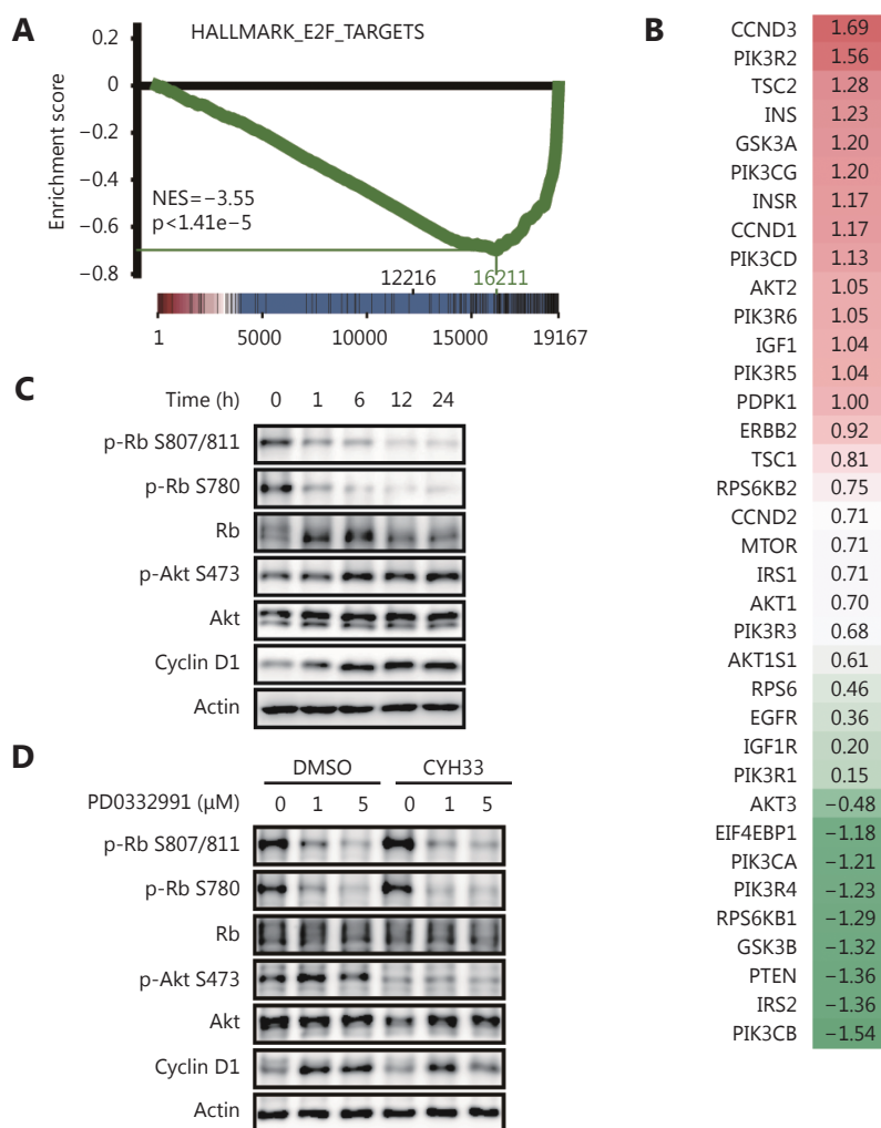
Figure 5 CYH33 abrogates PD0332991-induced AKT phosphorylation and cyclin D1 expression. (A, B) A549 cells were treated with vehicle or PD0332991 (1 \mu M) for 72 h and total RNA were extracted. Genome-wide gene expression profiling was performed by microarray analysis. (A) GSEA enrichment plot of differentially expressed genes in the gene set of Hallmark of E2F targets (HALLMARK_E2F_TARGETS) after treatment with PD0332991. (B) Heatmap of the mRNA levels of genes involved in the PI3K-AKT signaling pathway. The fold change (log 2) in the expression of the listed genes after treatment with 1 \mu M PD0332991 is shown. (C) A549 cells were treated with 1 \mu M PD0332991 for the indicated times and cell lysates were subjected to Western blot with the indicated antibodies. (D) A549 cells were treated with PD0332991 (0, 1 or 5 \mu M) alone or in combination with CYH33 (1 \mu M) for 72 h and cell lysates were subjected to Western blot with the indicated antibodies. Data are shown as representatives from at least three independent experiments.
