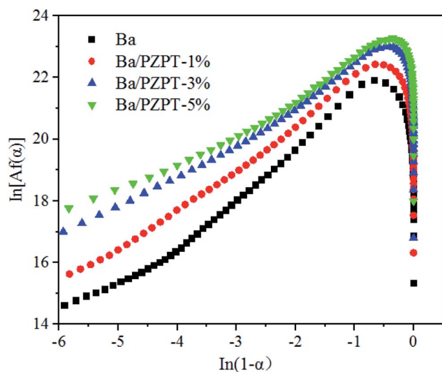
Fig. 6 Plots of \ln[Af(\alpha)] and \ln(1 - \alpha) of the Ba and Ba/PZPT systems at a heating rate of 5^\circ\text{C min}^{-1} by the average activation energy from Flynn–Wall–Ozawa method.
