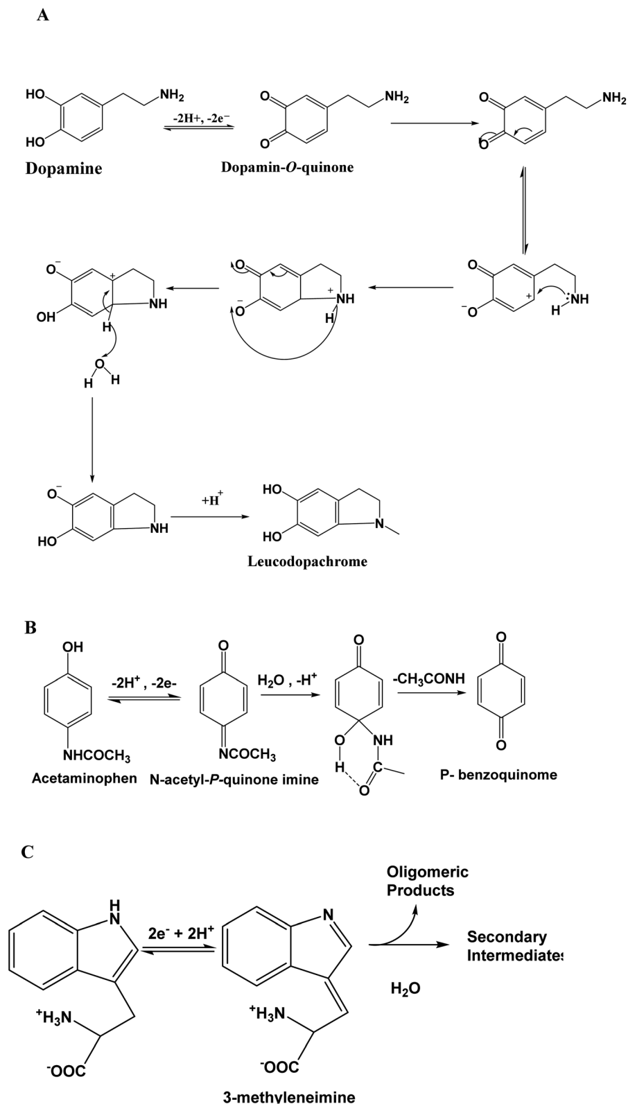
Scheme 1 Electrochemical reaction mechanism of (A) DA 39 , (B) AC 40 and (C) Trp. 41
