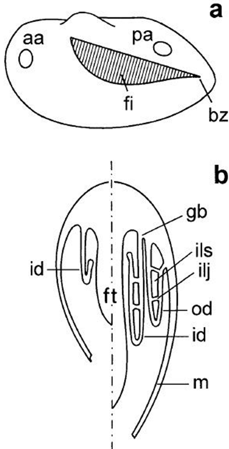
Fig 1. Diagram of gill position and cross-section through a lamella showing ascending and descending limbs of a filament. A: Gill position within a valve showing positioning of the anterior adductor (aa) and posterior adductor muscles (pa), budding zone (bz) and filaments (fi). B: A dorso-ventral section through a eulamellibranch showing the foot (ft), gill base (gb), inner demibranch (id), interlamellar junction (ilj), interlamellar space (ils), mantle (m) and outer demibranch (od). Used with permission from [38].
