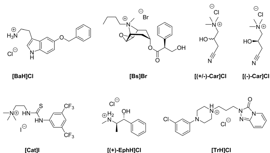
Fig. 1 Selected compounds (5-benzyloxytryptaminium chloride, butyl scopolaminium bromide, ( R,S )-carnitinenitrile chloride, ( R )-(-)-carnitinenitrile chloride, iodide salt of the catalyst, (1 S ,2 R )-(+)-ephedrine hydrochloride and trazodone hydrochloride) for crystallization and salt screening.
