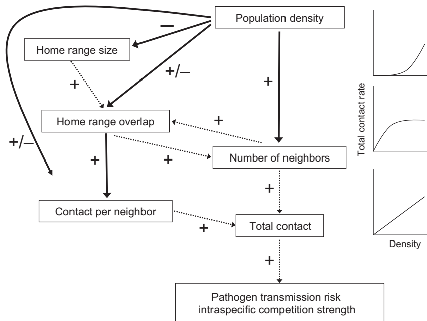
Figure 1. Possible pathways through which increases in density might influence contact rates, leading to accelerating, saturating, or linear relationships between density and contact rates. Solid lines indicate hypothesized pathways tested in this study. Dashed lines indicate pathways not directly addressed in this study.
