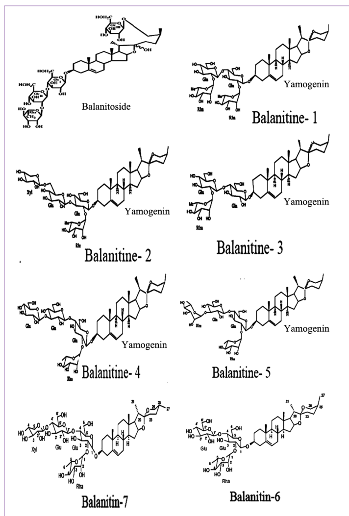
Figure 2: Chemical constituents of Balanites aegyptiaca
