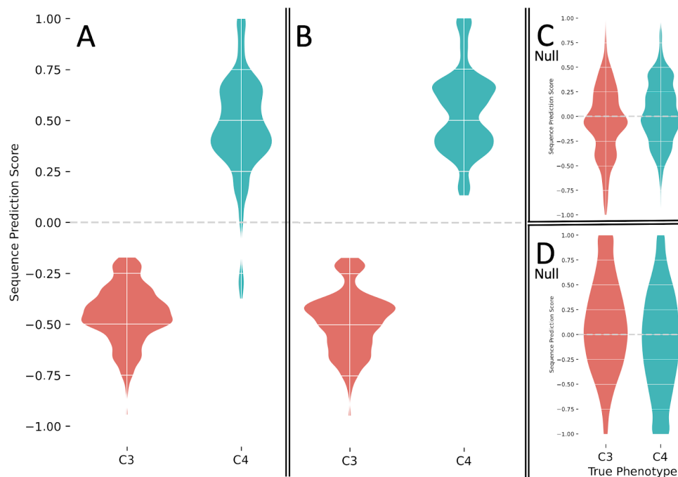
Figure 4. Predictive ability of ESL-PSC genetic models of C4/C3 photosynthesis. A-D Sequence prediction scores (SPS) from model ensembles are shown for known C4 (blue) and C3 (red) species in kernel density estimation plots. Negative SPS indicates a prediction of the C3 phenotype (trait-negative), and positive SPS indicates a prediction of the C4 phenotype. Predictions shown are for all species (A), species in clades independent of the clades contributing species for model training (B). Response-flipped null ESL-PSC models of C4/C3 photosynthesis (C). Null models were constructed by flipping the phenotype response values of 3 out of 6 of the input contrast pairs. This was done for all 10 distinct combinations of 3 out of 6 contrast pairs, and all model predictions were aggregated. SPSs from the best 5% of models by MFS are included. Pair-randomized null ESL-PSC models of C4/C3 photosynthesis (D). Null models were constructed by randomly flipping or not flipping the residues between each species contrast pair at every variable residue in the MSA. For each of the 25 alternative PSC input species combinations, randomized pair-flipped alignments were generated, and model ensembles were produced for each. Aggregated predictions are shown.
