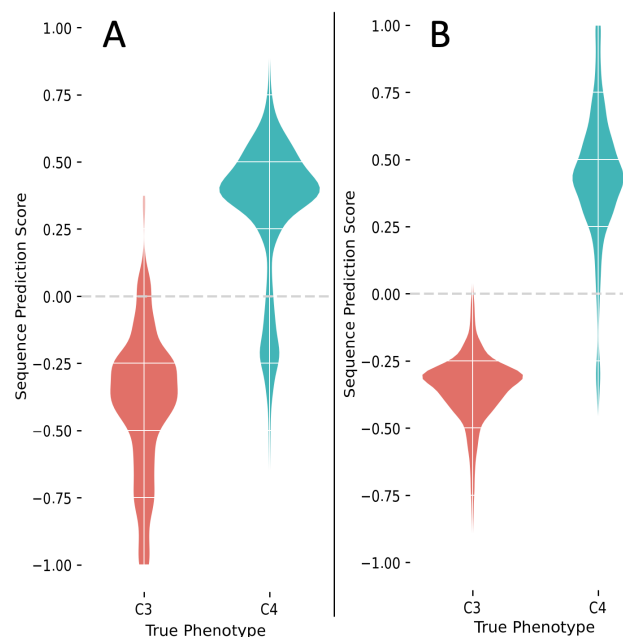
Figure 5. Alternative models. A: Predictions from models developed without the inclusion of RuBisCo are shown for independent species. B: Alternative PSC combinations. 100 alternative species combinations of PSC pairs were generated, and ensemble models were constructed as above. Predictions were aggregated for only the independent clades (black branches in Fig. 2). SPSs from the best 5% of models by MFS are shown from the aggregate of all ensemble models.
