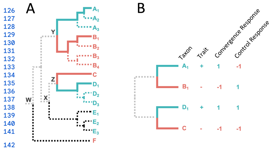
Figure 1. The paired species contrast (PSC) design. A: An example phylogeny with one set of selected species (solid blue and red lines). Extraneous lineages (black dotted lines) and shared evolutionary history (gray dotted lines). B: A schematic depiction of the four species selected for ESL-PSC analysis. In the ESL experiment, the response variable refers to the binary phenotype, where +1 represents the convergent trait, and -1 represents the ancestral trait.
