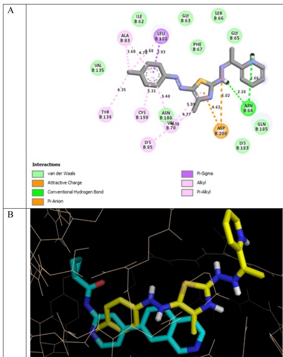
Fig. 12 (A) 2D binding interactions of compound 13a in GSK3 \beta (PDB ID 4PTE); (B) 3D structure of 13a (yellow) superimposed with 2WF (cyan) in GSK3 \beta (PDB ID 4PTE) in tint sticks.
