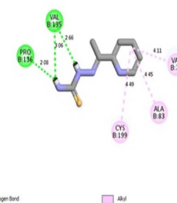
Fig. 14 2D binding interactions of compound 1a in GSK3 \beta (PDB ID 4PTE).
