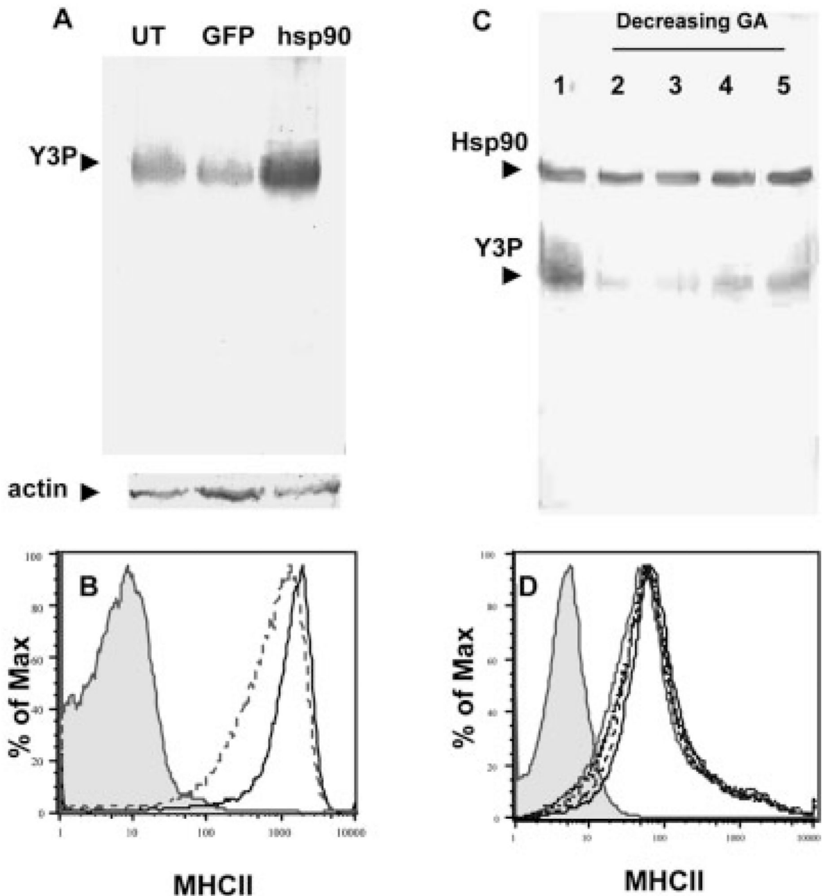
Figure 4. Hsp90 enhances SDS-stable MHCII heterodimer levels.
