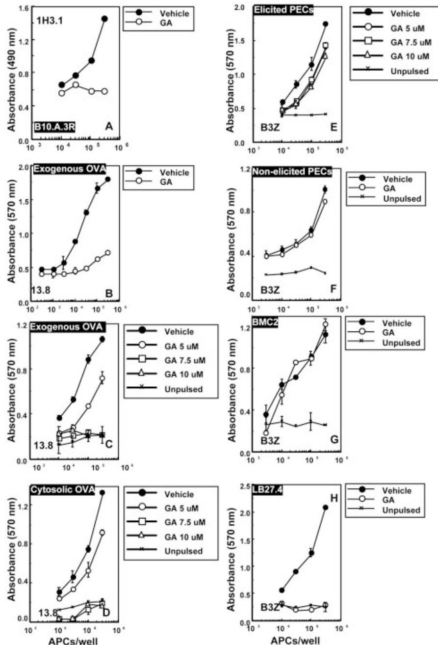
Figure 1. Geldanamycin inhibits MHCII-restricted presentation of endogenous and exogenous proteins.
