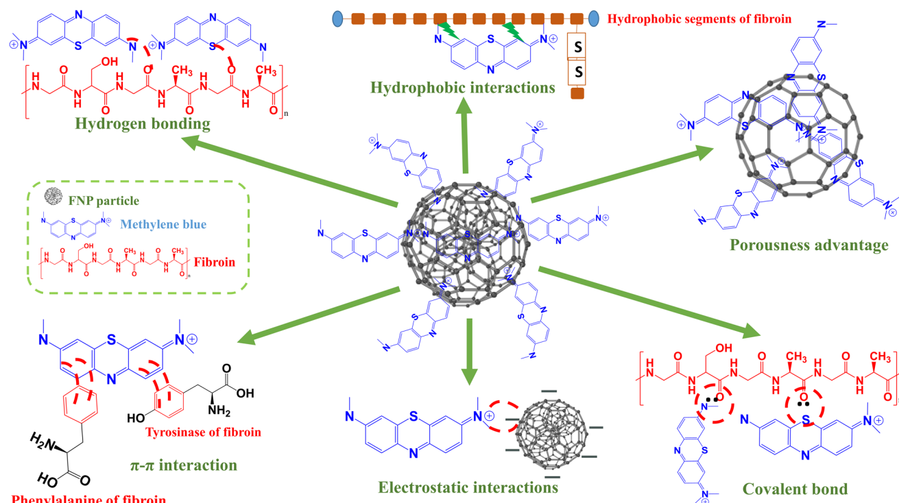
Fig. 7 MB adsorption mechanisms of FNP.
