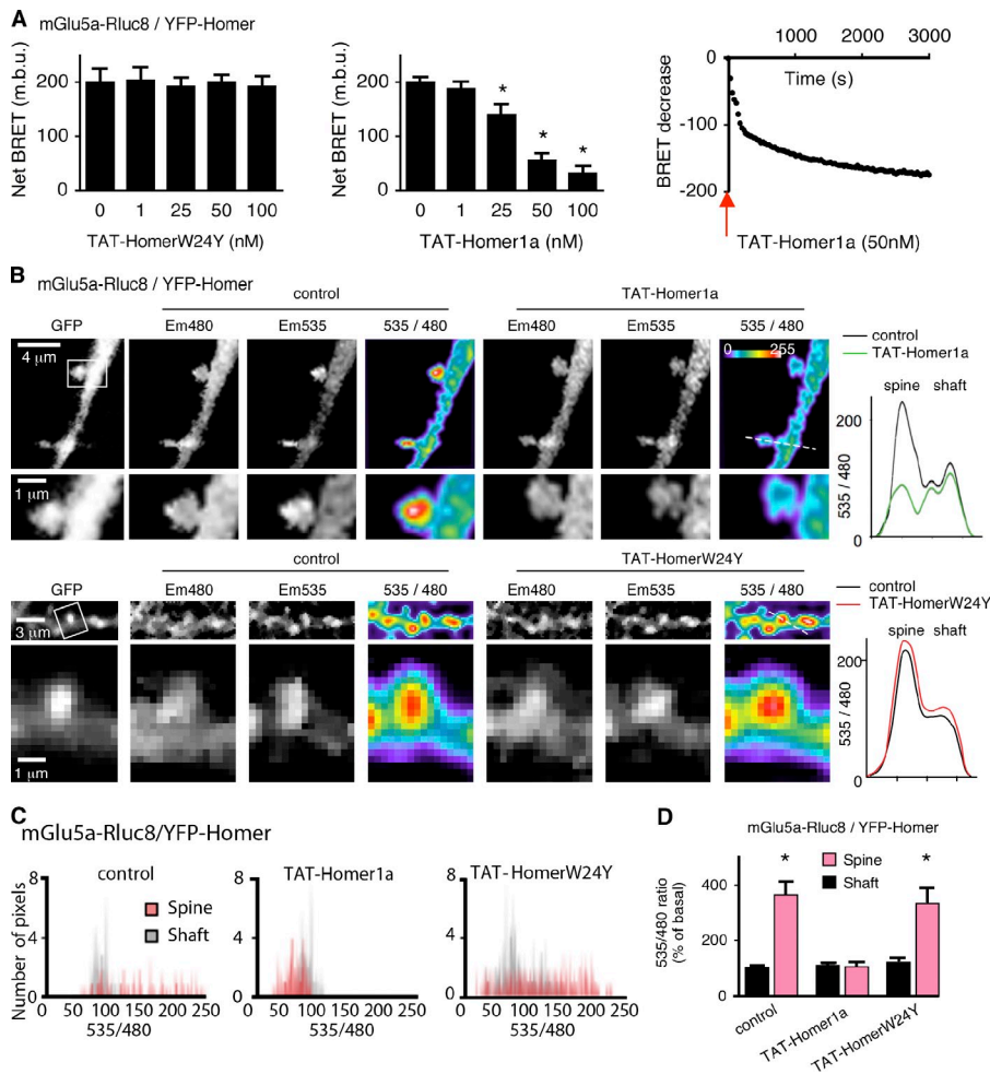
Figure 3. Homer1a disrupts the interaction between Homer and mGlu5a receptor in dendritic spines. (A) HEK293 cells were transfected with mGlu5a-Rluc8 and YFP-Homer. BRET signals were monitored 10 min after addition of the indicated concentrations of either TAT-HomerW24Y (left) or TAT-Homer1a (middle) and during 50 min in the presence of 50 nM TAT-Homer1a (right). The graphs show loss of interaction between mGlu5a receptor and Homer in the presence of TAT-Homer1a but not TAT-HomerW24Y (left, middle). This occurred in <5 min after the beginning of application to the TAT-Homer1a protein (right). The red arrow represents the application of the TAT-Homer1a protein. Each bar of histogram represents the mean \pm SEM of four experiments performed in triplicate. The asterisk represents significant difference from the BRET in absence of TAT. m.b.u., milli-BRET unit. (B–D) BRET images (B) and measurements (C and D) were obtained in neurons transfected with mGlu5a-Rluc8 and YFP-Homer before (control) and after exposure to TAT-Homer1a or TAT-HomerW24Y (50 nM; 10 min). (B) The pictures show expression of YFP-Homer (GFP), mGlu5a-Rluc8 (Em480), YFP-Homer excited by energy transfer (Em535), and BRET signals generated by the two tagged proteins (535/480). The right graphs indicate the profiles of the 535/480 ratio values along the dotted lines crossing the spine and shaft shown in the image before and after TAT-Homer1a or TAT-HomerW24Y perfusion. Bottom images show magnifications of the boxed areas. (C) BRET pixel distribution in spines and adjacent dendritic shaft regions ( n = 10 ) of a representative neuron before (control) and after perfusion of TAT-Homer1a or TAT-HomerW24Y. (D) Mean BRET intensity in the dendritic spine and shaft before (control) and during exposure to TAT-Homer1a or TAT-HomerW24Y. Each bar of the histogram represents the mean \pm SEM obtained from eight neurons and 7–10 regions/neuron. Note that in the presence of Homer1a, BRET signal between mGlu5a-Rluc8 and YFP-Homer decreased in spines but not the shaft. *, P = 0.05 .
