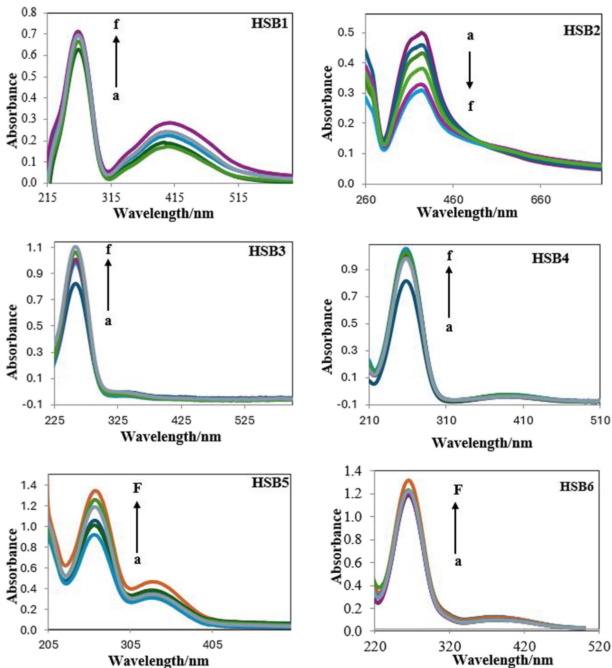
Fig. 4 UV-spectra of HSB1, HSB2, HSB3, HSB4, HSB5 and HSB6 ( 10 \times 10^{-6} mol dm -3 ) in the absence and presence of different concentrations of DNA at pH 7.4. Arrows show status of relative absorption intensity on incremental addition of different concentrations ( 1 \times 10^{-6} mol dm -3 ) of DNA (a) 0, (b) 1, (c) 2, (d) 4 (e) 5 (f) 5 into the constant concentration of each Schiff base under standard addition method.
