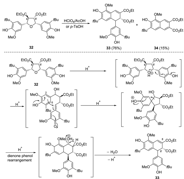
Scheme 9 Synthesis of ADHNs via acid-catalyzed cyclization of tetrahydrofuran.
