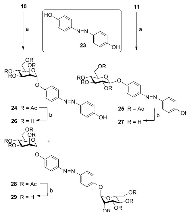
Scheme 3. Synthesis of azobenzene glycosides 26 , 27 , and 29 . a) \text{BF}_3 \cdot \text{Et}_2\text{O} , \text{CH}_2\text{Cl}_2 , 0^\circ\text{C} \rightarrow \text{RT} , 24 (37%), 25 (31%), 28 (31%); b) NaOMe, MeOH, RT, 26 (88%), 27 (89%), 29 (93%).
