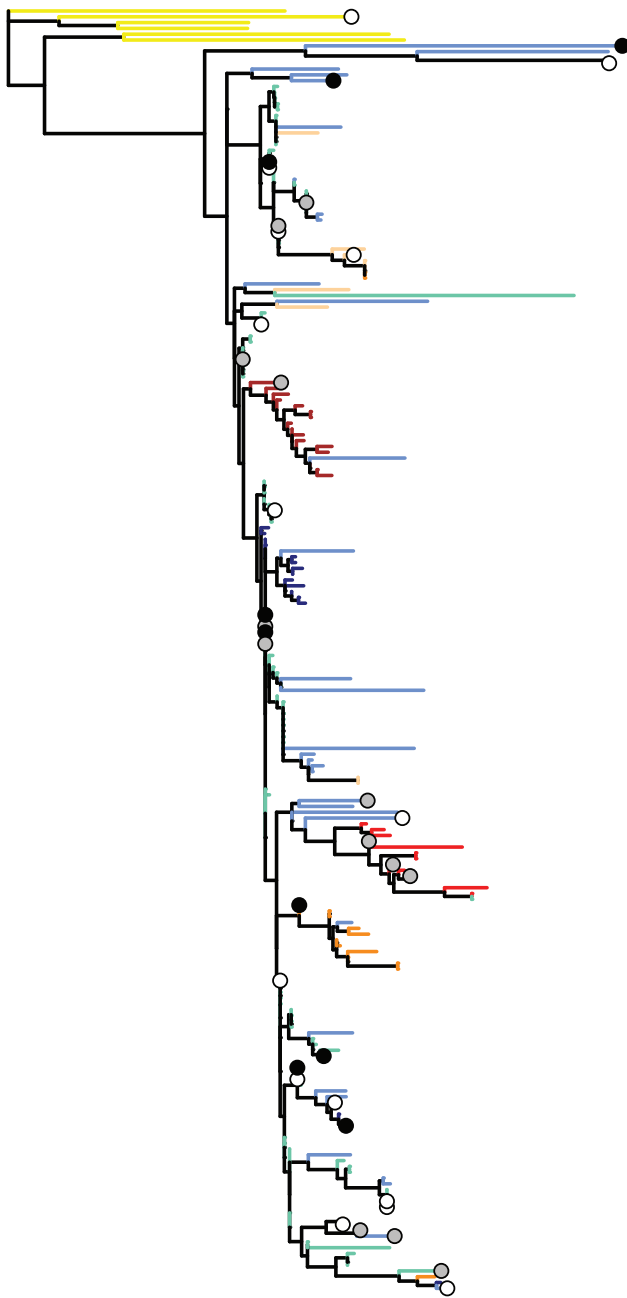
Fig. 3. —Phylogeny of SloEFV partial pol genes from extant and extinct sloth. The phylogenetic tree was calculated using RAxML; sequences from different sloth species are designated by color. Bootstrap support is indicated by circles 75–90 = white; 90–99 = gray; 100 = black. Sequences for pol genes were obtained for Bradypus variegatus (dark orange), Choloepus hoffmanni (dark blue), Choloepus didactylus (aquamarine), and Mylodon darwinii (red) by hybridization capture. Sequences for B. variegatus and Bradypus pygmaeus (light orange), C. hoffmanni (light blue) and M. darwinii (brown) were obtained in silico. Denoted in yellow are the pol gene sequences used as outgroups for tree construction: Bovine (NC_001831.1), Equine (NC_002201.1), Feline (NC_001871.1), Human (GenBank: Y07725.1), and Rhinolophus (GenBank: JQ814855.1) foamy viruses (all downloaded from NCBI).
