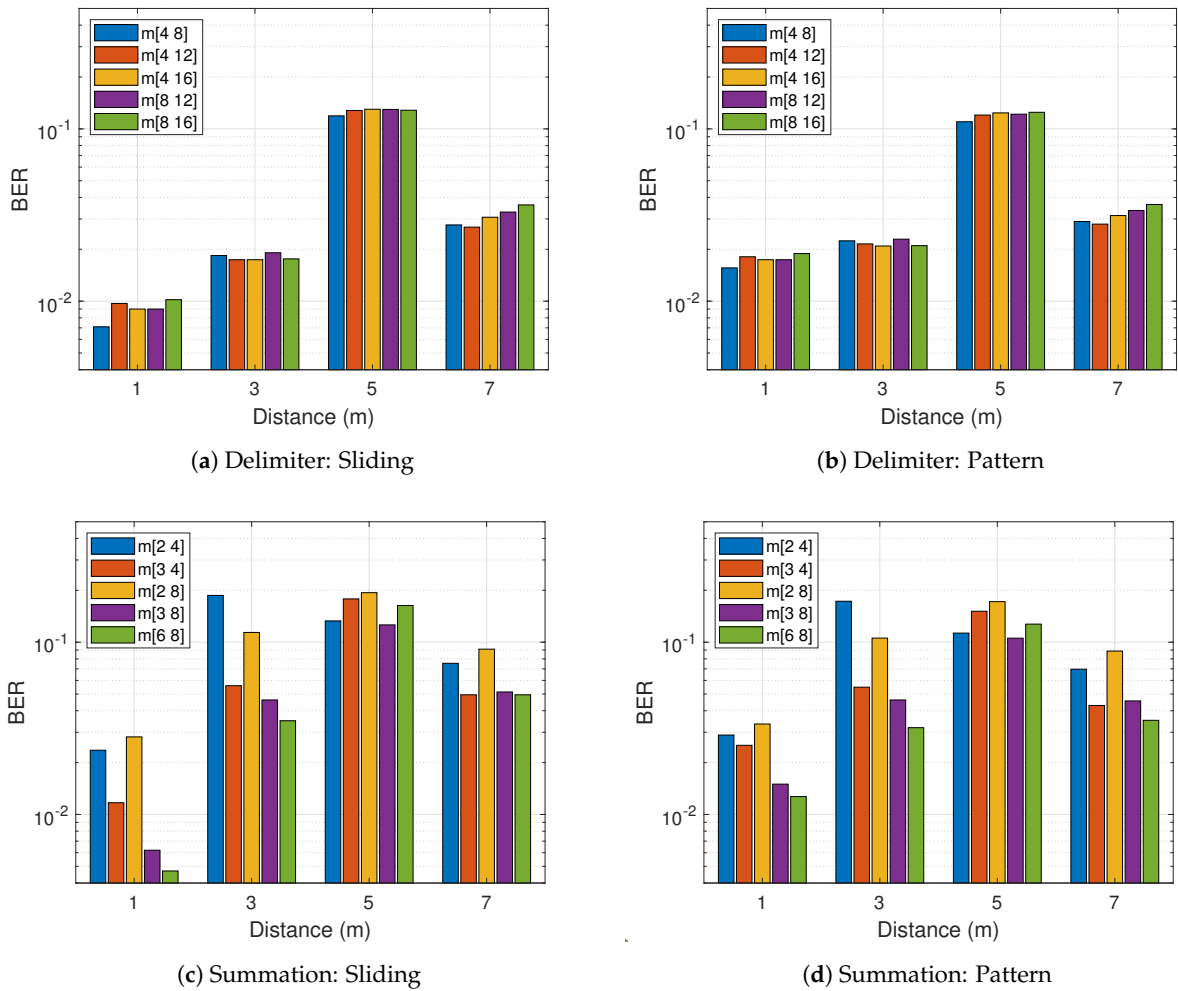
Figure 7. Experimental results for different filter constant m with sliding and pattern-based decoding.
