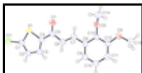
Fig. 1. ORTEP (Farrugia, 1997) view of the title compound, showing 50% probability ellipsoids and the atom numbering scheme.
