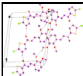
Fig. 2. A unit cell packing of the title compound showing intermolecular interactions with dotted lines. H-atoms not involved in hydrogen bonding have been excluded for clarity.
