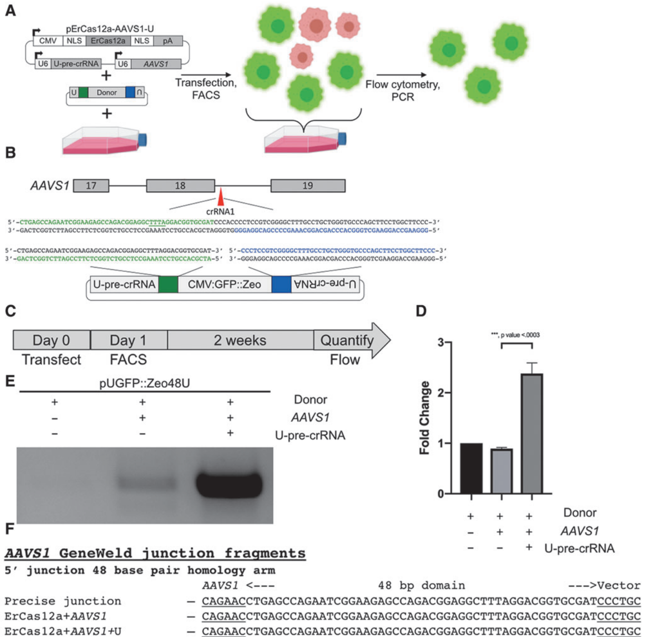
FIG. 6. Using ErCas12a for targeted integration in human cells. (A) Schematic showing the workflow for targeted integration at AAVS1 in HEK293T cells. (B) Schematic of AAVS1 showing designed homology for precise integration using ErCas12a and the U-pre-crRNA to liberate the cassette. Green block, 5' homology; blue block, 3' homology. The PAM for ErCas12a targeting in the genome and donor is underlined. (C) Schematic for flow analysis after transfection of GeneWeld reagents for targeting AAVS1 . (D) Bar graph showing the ratio of cells with GFP expression as determined by flow cytometry. Graph represents the mean \pm SD. p -Values calculated with one-tailed Student's t -test. (E) Junction fragment gel showing the expected 5' integration amplicon. No amplicon is seen when transfecting donor alone. (F) DNA sequencing of lanes in (E) showing a precise integration using the programmed homology.
