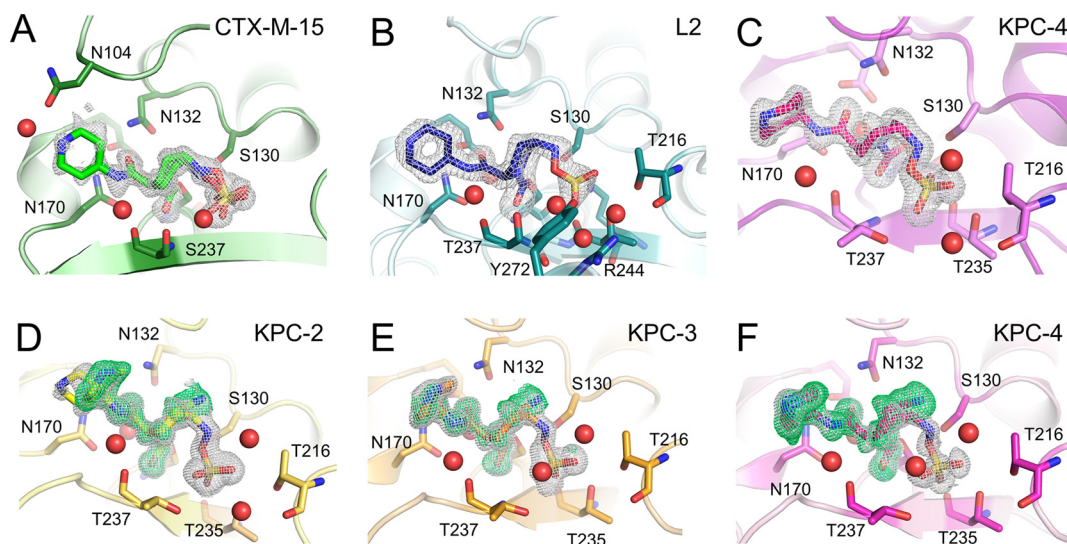
FIG 3 Electron density maps showing relebactam bound to the active sites of class A \beta -lactamases. Unbiased omit F_o-F_c electron density maps were calculated with the ligand removed and are shown contoured at 3\sigma . Gray density is calculated after removal of “intact” relebactam, green density after removal of desulfated relebactam. (A) CTX-M-15 (green, 16-hour soak), (B) L2 (teal, 16 hours), (C) KPC-4 (pink, 1 hour), (D) KPC-2 (yellow, 16 hours), (E) KPC-3 (orange, 16 hours), and (F) KPC-4 (16 hours).
