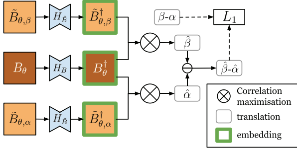
Fig. 10. The networks H_B and H_{\tilde{B}} are learned to project real live images and synthetic images to a joint embedding, where their translation offset can be found by maximizing correlation.
