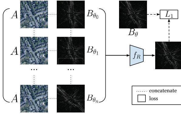
Fig. 6. Prior work in Tang et al. (2020b) proposes a network to infer the rotation offset. The rotation offset is found by softmaxing a stack of rotated radar images to produce a radar image with the same heading as the satellite image.
