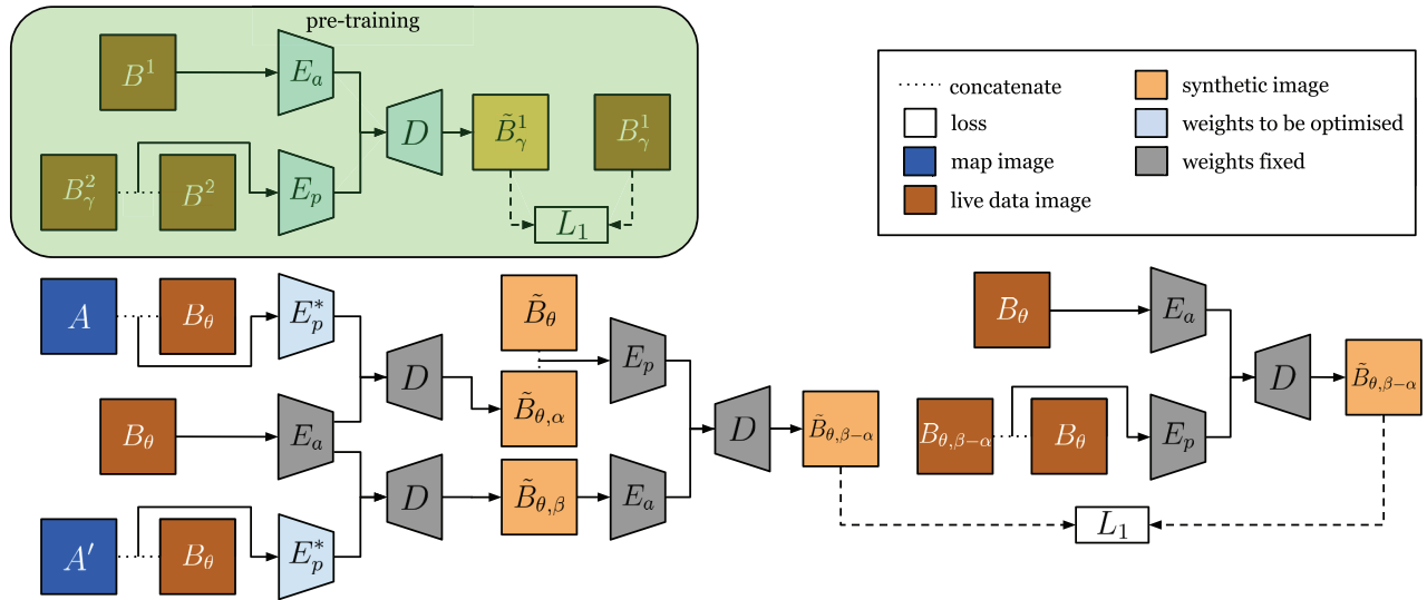
Fig. 9. Top: During pre-training, we can learn an appearance encoder E_a , and a pose encoder E_p that discovers the translation offset between an image of \mathcal{B} and a shifted version of itself. Bottom: Taking E_a , E_p , and D and fixing their weights, we seek to learn E_p^* which discovers the translation offset between two images from different modalities. Here E_a , E_p , and D can provide the necessary geometric and appearance relationships used for learning E_p^* self-supervised.
