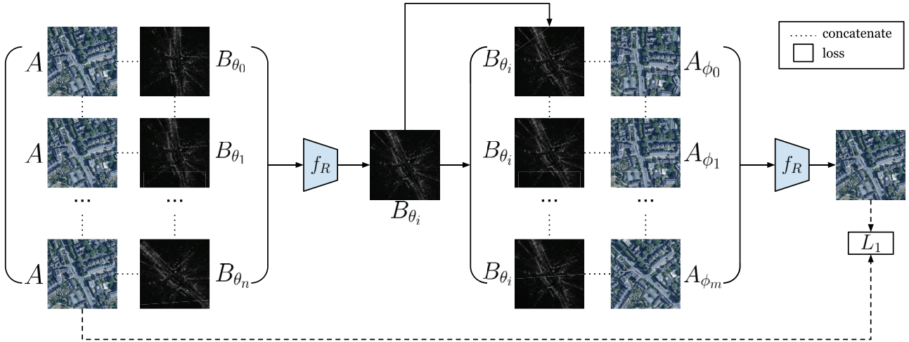
Fig. 7. Given A and a rotation stack \{B\} the network f_R finds B_{\theta_i} by taking softmax. Then, given B_{\theta_i} and a rotation stack \{A\} , the network outputs a softmaxed map image from \{A\} . A loss is applied to enforce the output of the second pass to be A , which in turn enforces the output of the first pass to be B_{\theta} . Here both symbols for f_R in the figure refer to the same network with the same parameters, but at different forward passes.
