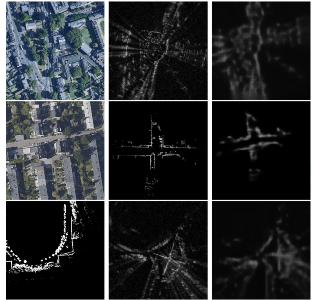
Fig 1. Given a map image of modality \mathcal{A} (left) and a live data image of modality \mathcal{B} (middle), we wish to find the unknown SE(2) offset between them. To do so, our method generates a synthetic image of modality \mathcal{B} (right) that is pixel-wise aligned with the map image, but contains the same appearance and observed scenes as the live data image. Top: localizing radar data against satellite imagery. Middle: localizing lidar data against satellite imagery. Bottom: localizing radar data against prior lidar map.
