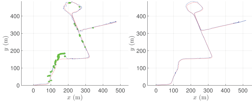
Fig. 13. Estimated pose (blue) versus ground-truth pose (red) for localizing a radar (left) and a lidar (right) against satellite imagery. Our system tracks the vehicle’s pose over 1 km, where we occasionally fall back to odometry for the radar experiment (green). Our system is stand-alone and requires GPS only for the first frame.
