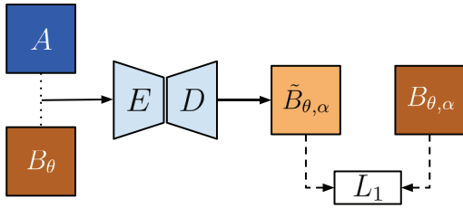
Fig. 8. Architecture for image generation in prior supervised approach (Tang et al., 2020b).
