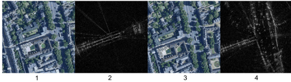
Fig. 4. Two radar images captured 15 seconds apart from each other (2 and 4), pixel-wise aligned with satellite images (1 and 3). Though the overlapping scenes in the satellite images are identical, the radar scans appear significantly different, as they capture different regions in their field of view.
