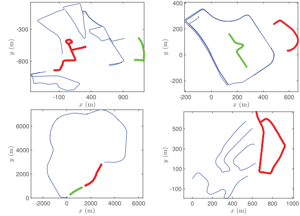
Fig. 12. Training (blue), validation (green), and test (red) trajectories for RobotCar (top left), KAIST (top right), Sejong (bottom left) and 20111003_drive0034 (bottom right). Certain data are removed to avoid overlap between the splits.
