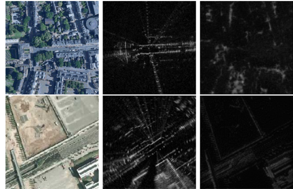
Fig. 5. Results of CycleGAN: satellite image (left), live radar image pixel-wise aligned with the satellite image (middle), synthetic radar image (right). There is no explicit constraint on which regions of the input satellite image will appear in the output synthetic image. As a result, this leads to large localization error as the synthetic image does not contain scenes observed by the live radar image.
