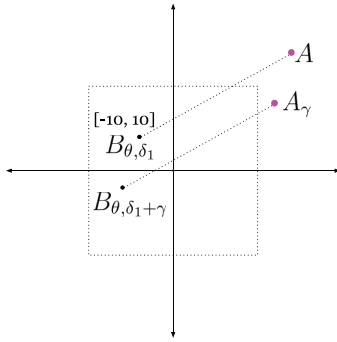
Fig. 19. The resulting synthetic image will still be erroneous, if an incorrect quadrant is selected. Here the offset between B_{\theta, \delta_1} and A is larger than what the networks can handle. In this case, generating \tilde{B}_{\theta, \alpha} and \tilde{B}_{\theta, \alpha + \gamma} will both be problematic due to the issue with offsets.
