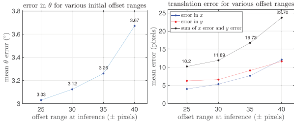
Fig. 15. Mean error in rotation (left) and translation (right) with larger initial translation offset range, evaluated for radar localization against satellite imagery on the RobotCar Dataset.
