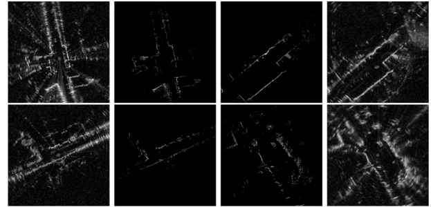
Fig. 20. Qualitative results of CycleGAN for domain adaptation between a single scan of radar and lidar data. From left to right: a real radar image and its synthetic lidar image, a real lidar image and its synthetic radar image. Top: CycleGAN applied in Cartesian coordinate representation. Bottom: CycleGAN applied in polar coordinate representation.
