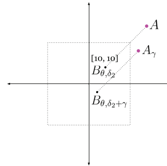
Fig. 18. If we shift B_\theta by [10, 10] to form B_{\theta, \delta_2} , then the offset between A and B_{\theta, \delta_2} is within what the networks are designed for. In this case, generating \tilde{B}_{\theta, \alpha} and \tilde{B}_{\theta, \alpha + \gamma} should both be accurate, as the offset in both cases are within what the networks are trained for.
