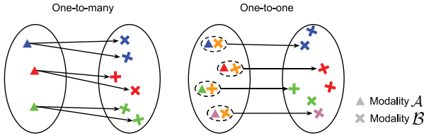
Fig. 3. A one-to-many mapping (left) versus a one-to-one mapping (right). Left: the mapping from modality \mathcal{A} to modality \mathcal{B} preserves color, but is ambiguous in orientation of the output, resulting in a one-to-many mapping, and is therefore not a function. Right: augmenting the input with an element of \mathcal{B} offers additional constraint in orientation, resulting in a one-to-one mapping as the mapping is now unambiguous in both color and orientation. Note that the mapping on the right is one-to-one, but not necessarily surjective .
