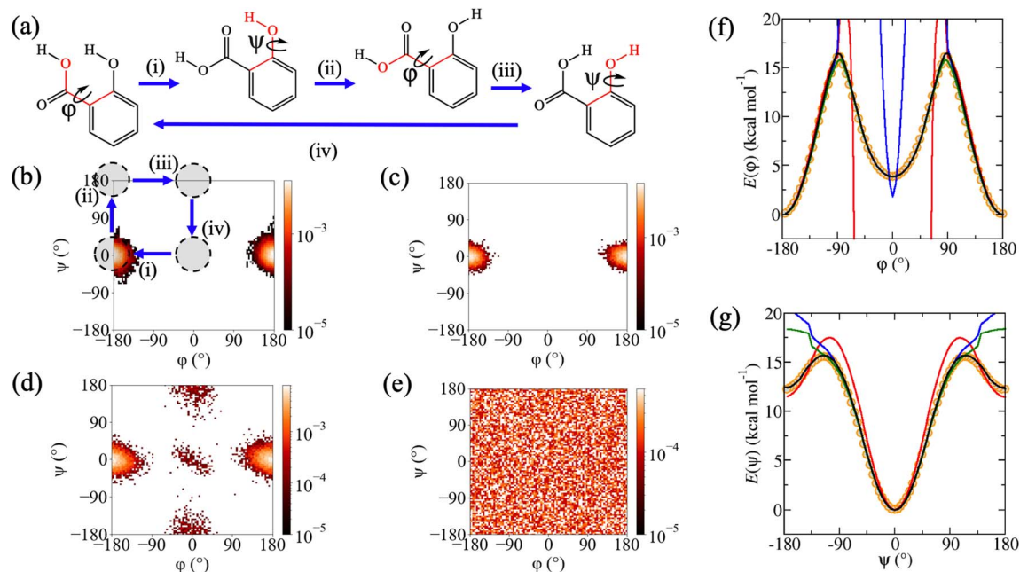
Fig. 4 (a) Key conformational transitions (i)–(iv) of salicylic acid defining the (\varphi, \psi) -surface. Relative population densities of the (\varphi, \psi) -surface for the (b) rMD17, (c) MD-300K, (d) MD-500K and (e) Meta-300K datasets with conformational transitions (i)–(iv) highlighted in (b). For rMD17, the populations were calculated using all 10^5 structures in the dataset. Energy profiles with respect to torsional rotation around (f) \varphi , and (g) \psi , obtained from B3LYP-D3/6-31G* calculations (orange circles) and predicted from MLPs trained on rMD17 (red lines), MD-300K (blue lines), MD-500K (green lines) and Meta-300K (black lines) datasets.
