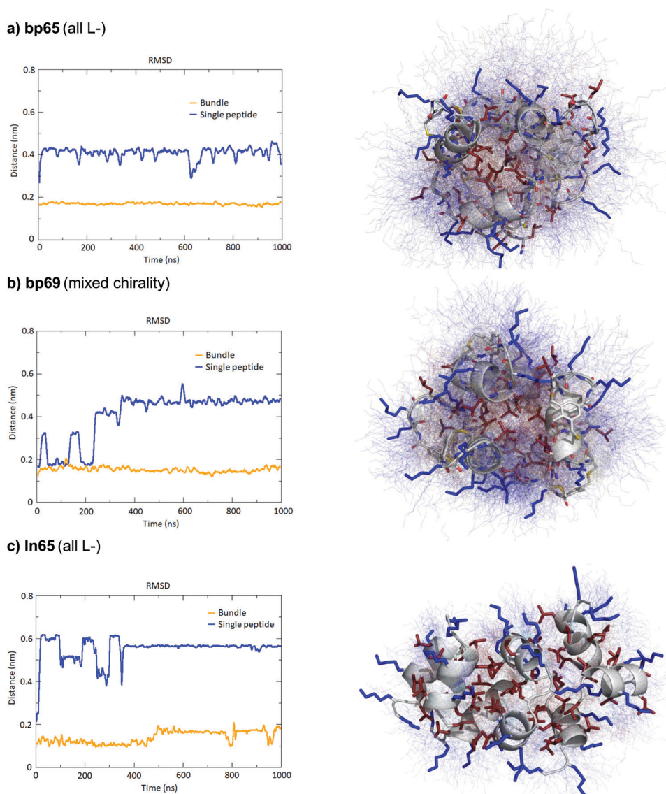
Fig. 5 MD simulations of helix bundles for bp65 , bp69 and ln65 from X-ray structures of bp65 , bp71 and Fdln65 . (a) MD simulations of bp65 as a bundle. Left panel: Root mean square distances of the backbone atoms relative to the backbone atoms of the starting model of a single peptide in the bundle compared to single peptides in water. Right panel: Overlay of 100 states over the 1000 ns run trajectory of the bundle in water. The average structure is shown as cartoon (backbone) and sticks (sidechains) and the 100 states as thin lines. Hydrophobic side chains are colored in red and cationic side chains in blue. (b) Same as (a) for bp69 for the bundle containing three complete peptides in the bundle out of four. (c) Same as (a) for ln65 . All fucoses were removed before simulations.
