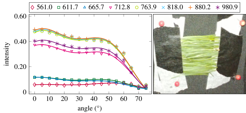
Figure 5. The plotted incidence angle versus laser backscatter intensity for the pine needles, abaxial side. The second-order Fourier series approximation fitted to the data is also shown for all wavelengths. (Online version in colour.)
