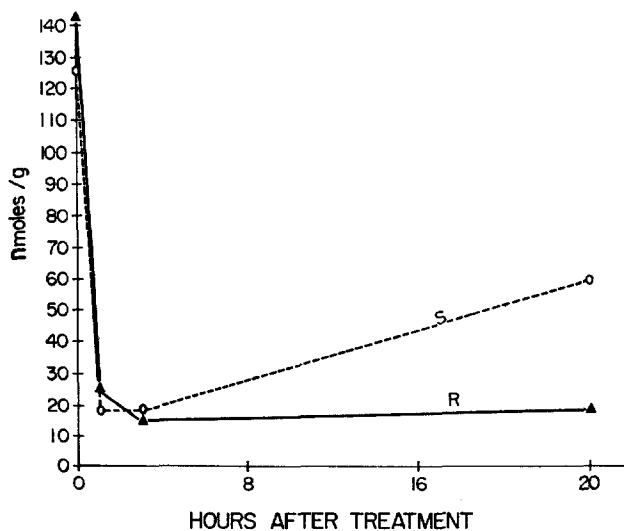
FIG. 2. Free asparagine content of 6C3HED tumors treated with L-asparaginase. Subcutaneous tumors were used 8-9 days after implantation of mice with approximately 2 million lymphoma cells. After careful blotting on gauze they weighed approximately 500 mg each. "S" indicates the asparaginase-sensitive tumor and "R" the resistant variant. For measurement of asparagine content at 1 and 3 hr, 1.0 ml agouti serum (360-420 units) was given intravenously. The number of animals used and standard deviations were: 1 hr, S-(11) \pm 1.03; R-(4) \pm 1.10. 3 hr, S-(4) \pm 0.21; R-(4) \pm 1.14. For measurements after 20 hr treatment, asparaginase was given intraperitoneally.
