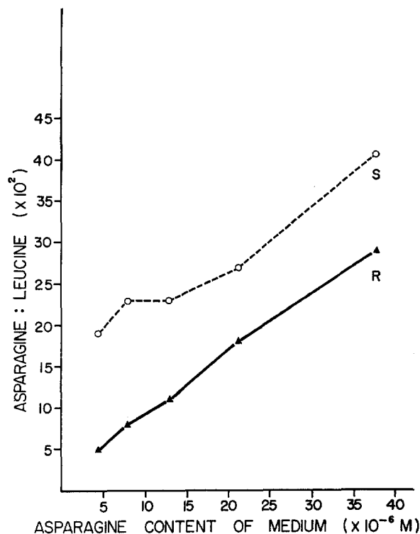
FIG. 5. Ratio of exogenous asparagine to leucine in proteins of Lymphoma 6C3HED.
