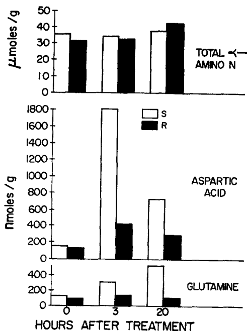
FIG. 7. Effect of L-asparaginase treatment on amino acid levels in 6C3HED tumors. Experimental animals were treated as described in Fig. 2, with 1.0 ml agouti serum (340 units). Total free \alpha -amino nitrogen was measured by the ninhydrin reaction (27) on picric acid supernatants used for assay of asparagine and other amino acids. Results in each case represent averages of three to six experiments.
