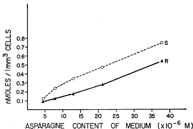
FIG. 3. Incorporation of exogenous asparagine into proteins of Lymphoma 6C3HED. Method as described earlier, measuring incorporation in 1 hr of incubation. With resistant cells (see reference 12) the rate of incorporation is linear in the 1st hr of incubation. With sensitive cells when low asparagine concentration limits utilization, the rate decreases after the first 10 min.
