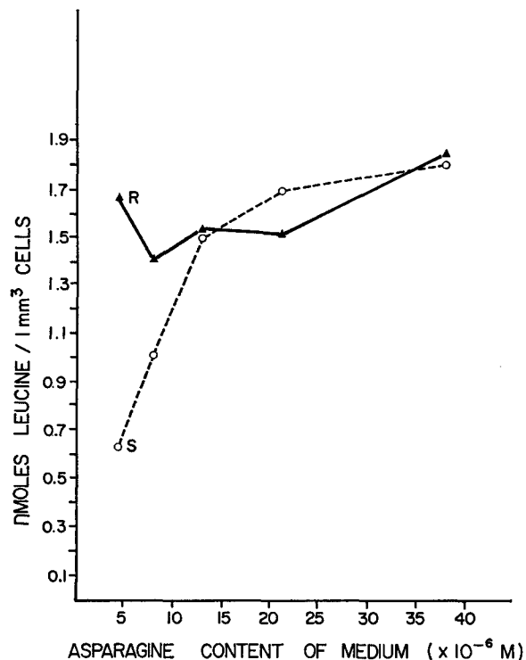
FIG. 4. Incorporation of exogenous leucine into proteins of Lymphoma 6C3HED.
