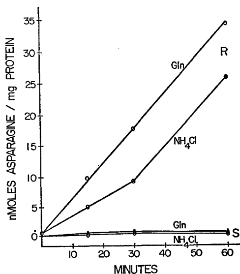
FIG. 6. Asparagine synthesis by pH 5 enzyme of cells of Lymphoma 6C3HED. Lymphoma cells were suspended in 5 volumes of 0.35 M-buffered sucrose (solution A, reference 25) and lysed by three cycles of freezing and thawing. The suspension was centrifuged at 12,000 g for 30 min, the supernatant diluted with 3 volumes of sucrose solution B and centrifuged at 120,000 g for 120 min. The supernatant from this stage was brought to pH 5.2 with dilute acetic acid and the precipitate which formed was centrifuged down at 10,000 g for 10 min. The precipitate was dissolved in glutathione- versene -tris buffer (pH 7.5) according to Patterson and Orr (24), and kept frozen at -20^{\circ}\text{C} till use. In assays the incubation mixtures consisted of 1.0 ml 1.5 \times 10^{-3} M L-aspartic acid with 0.25 \mu\text{C} L-aspartic acid -^{14}\text{C} [UL] (New England Nuclear Corp.), 2 \times 10^{-2} M L-glutamine (or 3 \times 10^{-2} M \text{NH}_4\text{Cl} ), 1 \times 10^{-2} M potassium ATP (Mann Research Laboratories, Inc.), 1 \times 10^{-2} M magnesium chloride, 0.1 M Tris, final pH 8.0. 0.2 ml enzyme preparation was added to this. The reaction was stopped by heating aliquots in a boiling water bath for 2 min. Asparagine and aspartate were separated by high voltage electrophoresis at pH 6.5, the location of each was determined by radioautography, and radioactivity on the paper was measured by liquid scintillation counting. Protein was estimated by a modification of the Lowry method (26).
