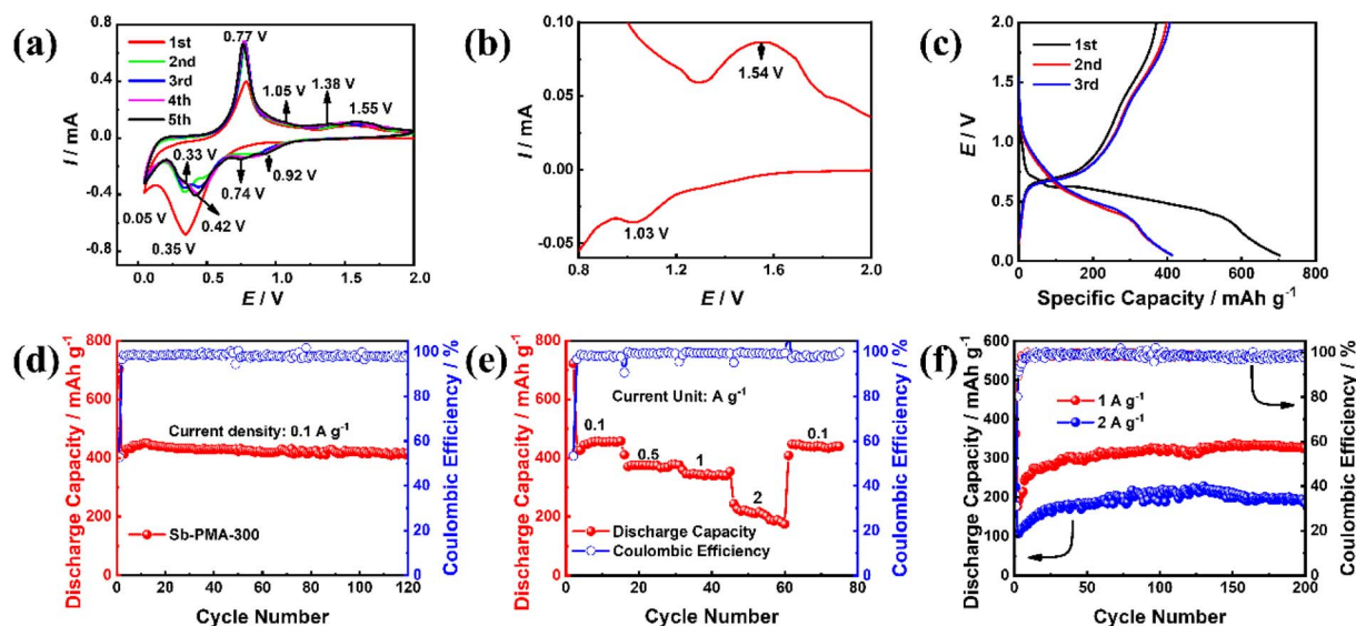
Fig. 4 Electrochemical properties of Sb-PMA-300: (a) the first five CV curves at 0.2 \text{ mV s}^{-1} , (b) partial amplification of the first CV curve in (a), (c) the first three charge and discharge profiles at 0.1 \text{ A g}^{-1} , (d) cycle performance at 0.1 \text{ A g}^{-1} , (e) rate capability, and (f) cycle performance at 1 \text{ A g}^{-1} and 2 \text{ A g}^{-1} .
