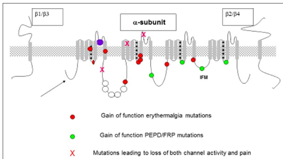
Figure 1. Voltage-gated sodium channels – human Na_v1.7 pain-related mutations (Emery et al. 2016).
