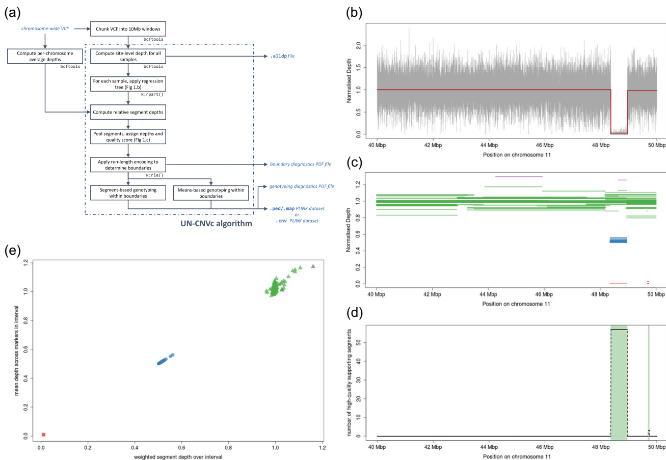
FIGURE 1 Overview of the UN-CNVc algorithm. (a) Overview of the pipeline, with input and output files in blue, and external tools and libraries in grey. (b) Output of a piecewise constant regression (in red) on a 10Mb window on chromosome 11, for a homozygous deletion carrier. The gray signal is the raw relative depth at every sequenced marker for that sample. (c) Pooled regressed segments across the population, with colour indicating the attributed ideal depth (0: red, 0.5: blue, 1: green, and 1.5: purple). (d) Raw count (dashed line) and run-length encoding (shaded green bars) on the number of high-quality segments with ideal depth < 1 . (e) Genotyping using both weighted average segment depth (colour, scheme identical to c) and average depth across markers (plotting glyphs, squares: 0, circles: 0.5, and triangles: 1). UN-CNVc, Unimaginatively Named CNV caller
