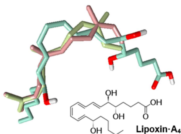
Figure 4. Chemical structure of lipoxin A 4 and alignment of lipoxin-A 4 (green), ( E,E )- \alpha -farnesene (pink), and ( Z,E )- \alpha -farnesene (khaki).
