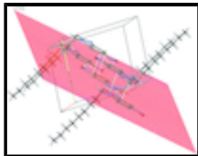
Fig. 2. Partial packing view of the title compound, showing tapes in the (-1 2 2) plane, built up from molecules linked through N—H...O hydrogen bonds and intermolecular C—H...O contacts (dashed lines).
