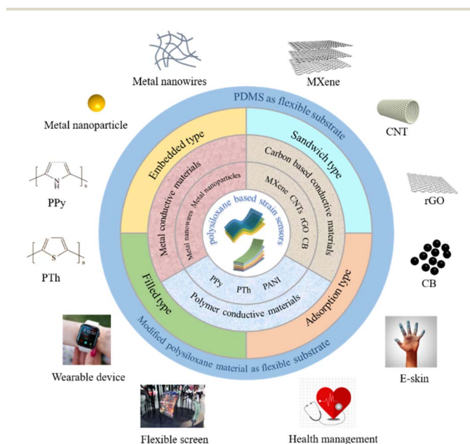
Fig. 1 Overview of several typical polysiloxane-based piezoresistive flexible human electronic sensors.
