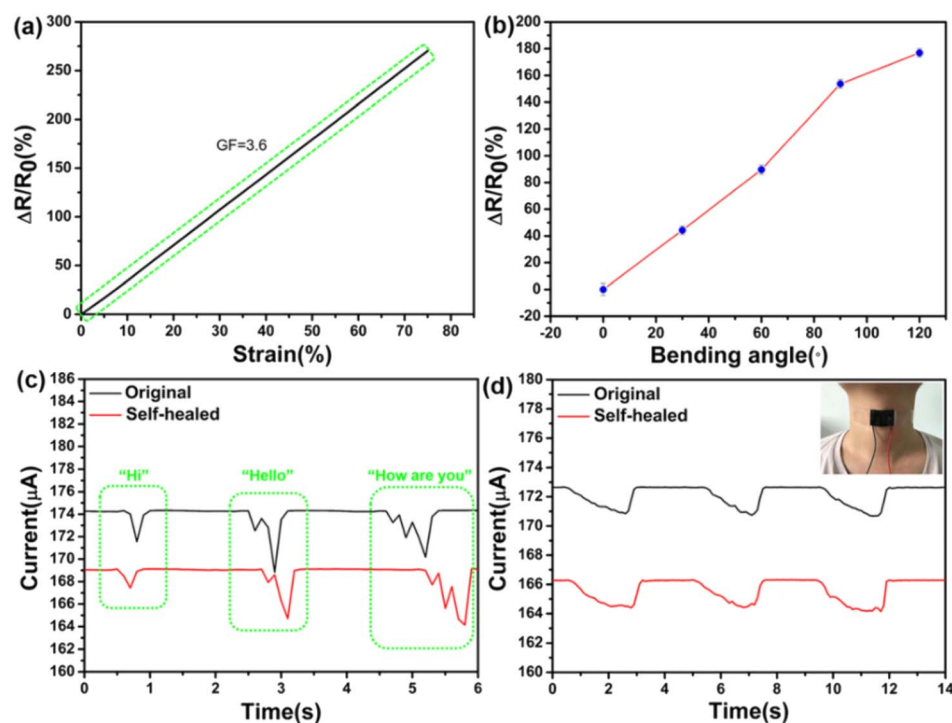
Fig. 25 (a) Relative resistance change of the MXene/PDMS flexible sensor during stretching; (b) relative resistance change of the MXene/PDMS flexible sensor when the elbow is bent; (c) current change of the MXene/PDMS flexible sensor when recognizing different words; (d) current change of the MXene/PDMS flexible sensor during swallowing 93 (Copyright 2020, The American Chemical Society).
