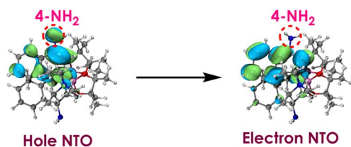
Fig. 1 Natural transition orbital (NTO) pair for S_1 excited state for 4-amino derivative.
