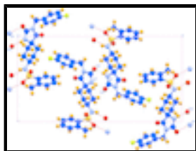
Fig. 2. A view of the crystal structure down the a axis. Dashed lines indicate hydrogen bonds.
