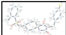
Fig. 1. The molecular structure with displacement ellipsoids drawn at the 50% probability level. The H atoms are shown as spheres of arbitrary radius. The dashed lines indicate the intramolecular hydrogen bond.
