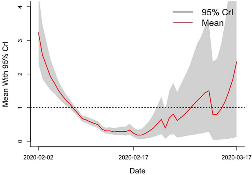
Figure 1. Daily R_{eff} curve in Wuhan, China
