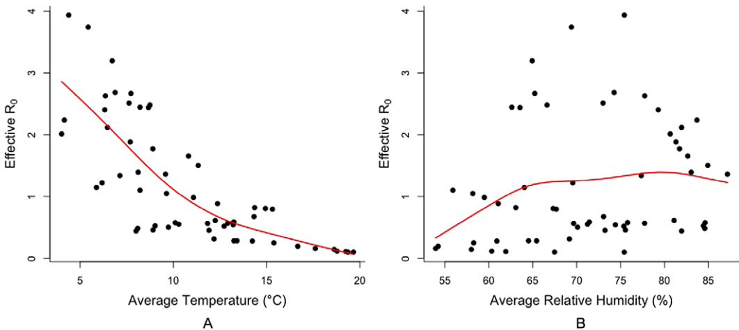
Figure 2. The smoothing spline with 4 degrees of freedom between daily R_{eff} and TEMP (panel A); daily R_{eff} and RH (panel B).
