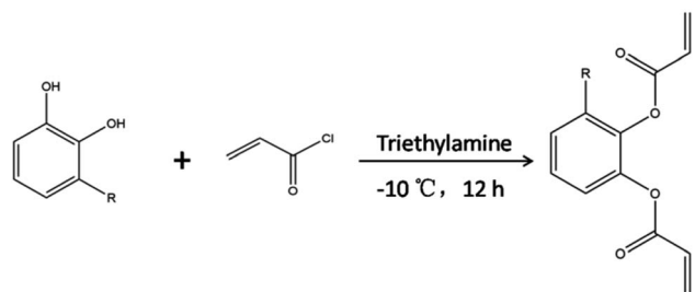
Fig. 3 Synthetic route of the urushiol derivative.
